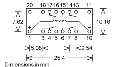
CEPHOS C-TQ4 Relay Module (4 x Form C) Top View
